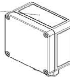
3G CELLULAR STRIP ANTENNA UNDER THIS SURFACE
