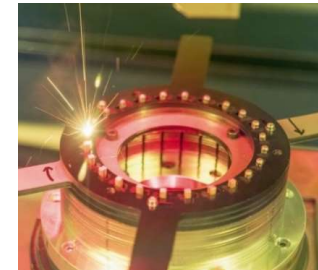
Gehring; Hairpin- Technology, Quantum
