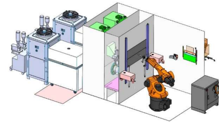
Chiron; Laser-cladding, Quantum HV
